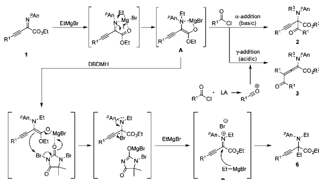
Scheme 3. Plausible Mechanism
