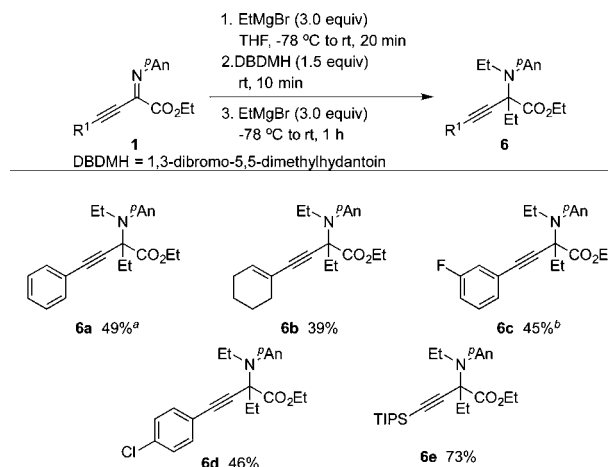
Scheme 2. Tandem N,C -Diethylation via an Iminium Salt
